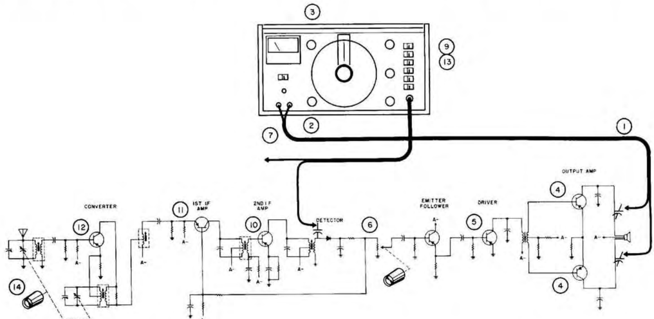
Figure 7. Typical Troubleshooting Technique Using RF Signal Generator
