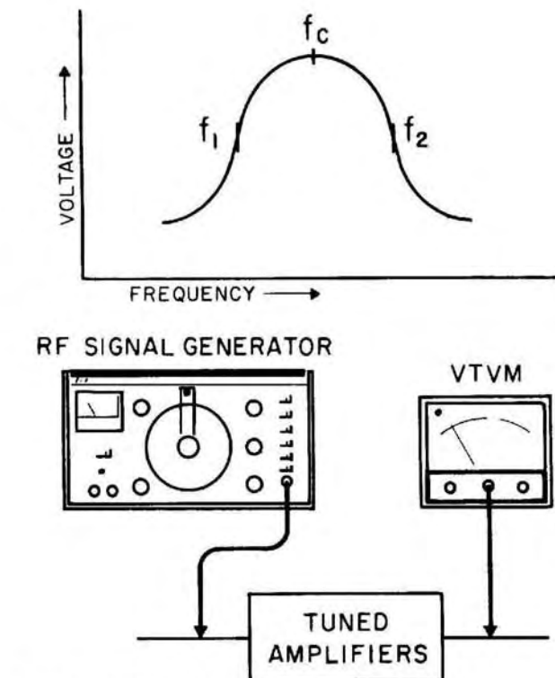
Figure 8. Making Gain Measurements
