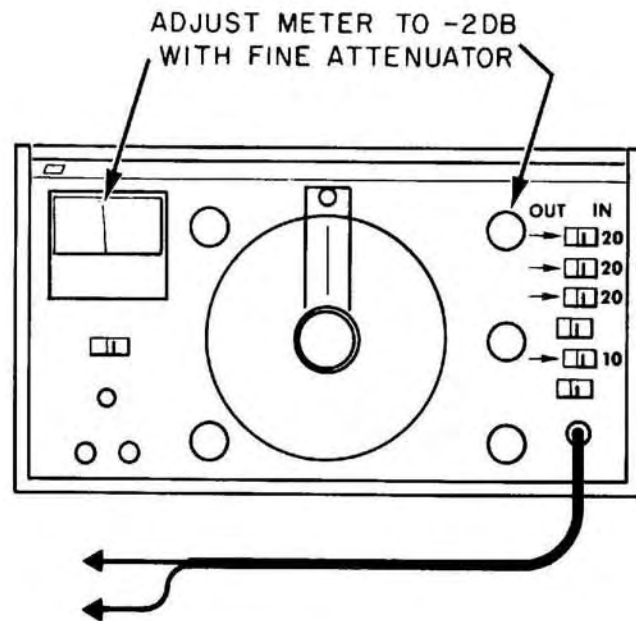
Figure 2. Typical Example, Setting Signal Level
