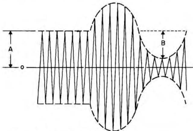
Figure 3. Amplitude Modulation Percentage
