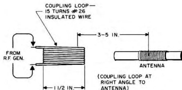
Figure 5. Signal Injection Coupling Loop for Ferrite Loopstick Antenna
