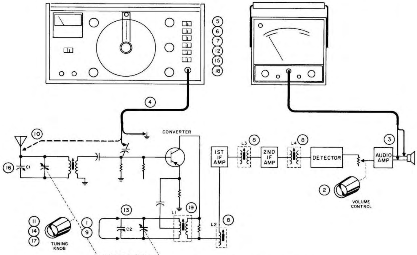
Figure 4. Typical AM Broadcast Band Receiver Alignment
