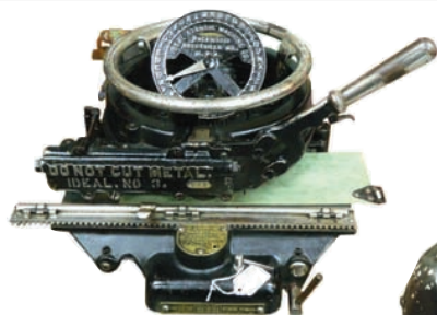
Ideal Stencil Machine Co., circa 1915, $275. DLR DH.
