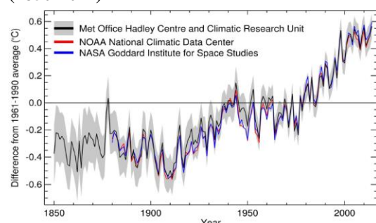
Global average temperature anomaly (1850-2014)
