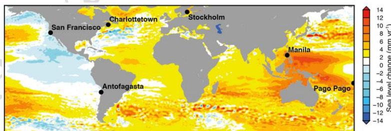
Figure 42 Observed sea level rise from 1993–2012
