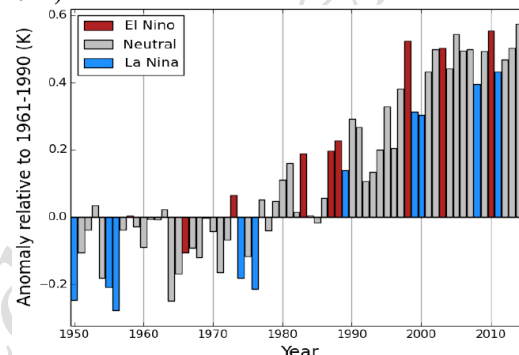
Global average temperature anomaly (1950-2014)
