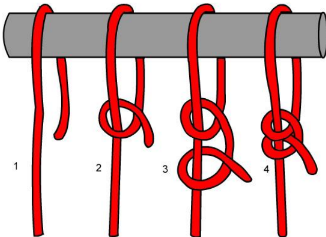
2 half-hitches
