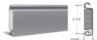
Flat Slat F2.5 - Polystyrene / R-value= 4.7
