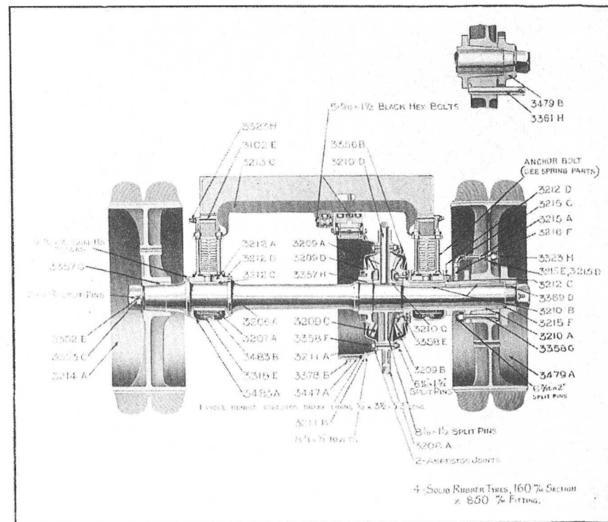
Rear Axle for 6 Ton Waggon (continued)
